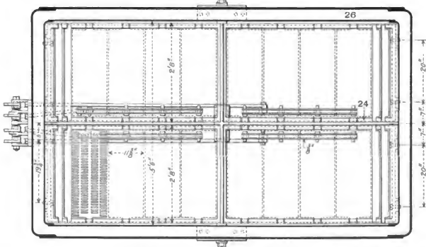
Figs. 525-527. Gate for Six-Wheel (0-6-0) Switching Locomotive with Wide Firebox. Erie Railroad.
